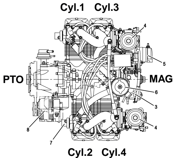
Figure 2: Cylinder arrangement
