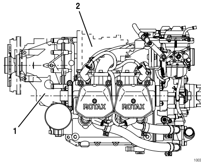
Figure 1: Engine components
