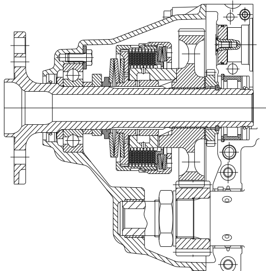
Figure 8: Overload clutch
